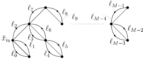
Fig. 1. The path \ell = \{\ell_0, \dots, \ell_{M-1}\} introduced in the proof of Lemma 3.4.
